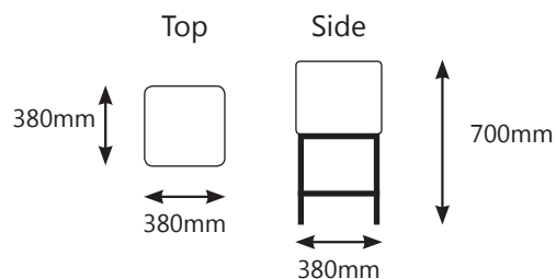
CRAZE BAR STOOL DIMENSIONS
