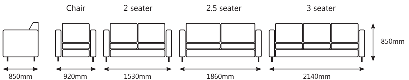
FRANKFURT DIMENSIONS
