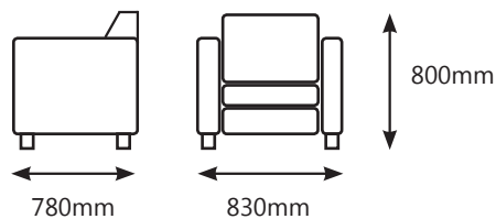
NURSING CHAIR DIMENSIONS
