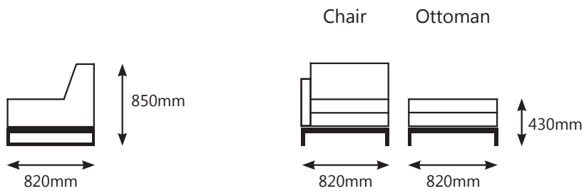
PLAZMA DIMENSIONS
